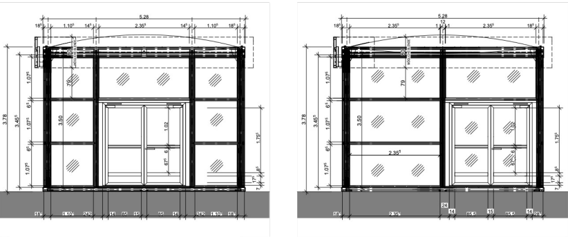
FASSADEN MANHATTAN CUBE 5X5 METER
