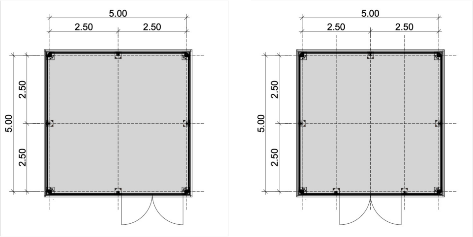
GRUND RISSE MANHATTAN CUBE 5X5 METER
